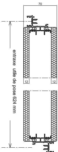
Cassette Danpatherm Fig. 1
